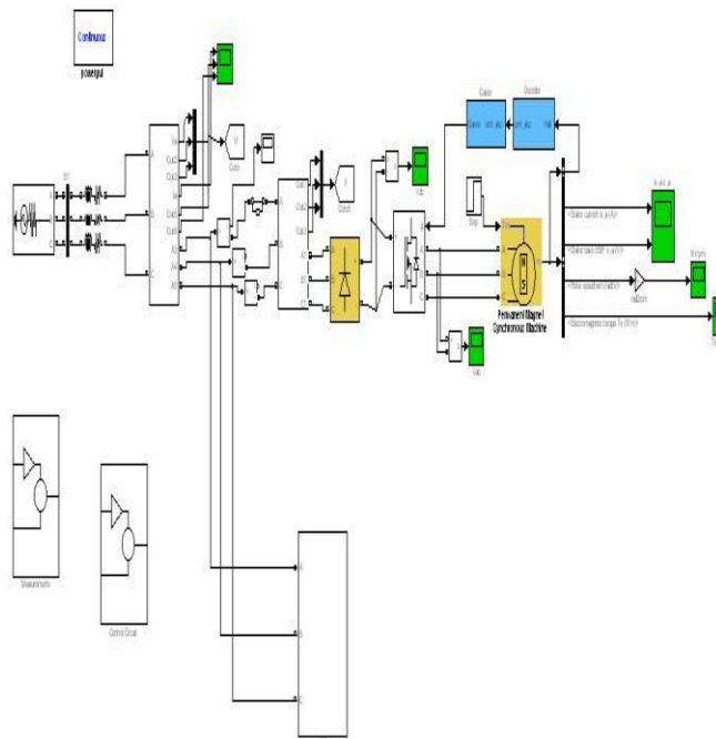
Figure. 8 Matlab/Simulink model of APF BLDC Drive
