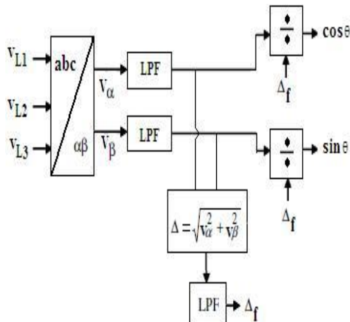
Figure.5 Principal of modified (id-iq) method
