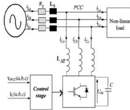
Figure. 1 Basic principal of shunt current compensation in active filter
