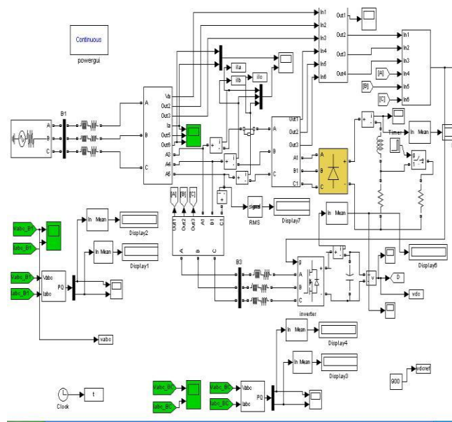
Figure.6 Matlab/Simulink Model of Shunt Active Power Filter
