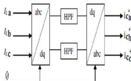
Figure.4 Principal of the synchronous reference frame method
