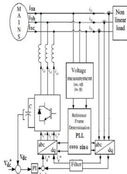
Figure. 3 Basic principle of SRF
