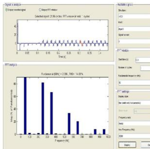
Figure. 11 FFT analysis of source current without APF
